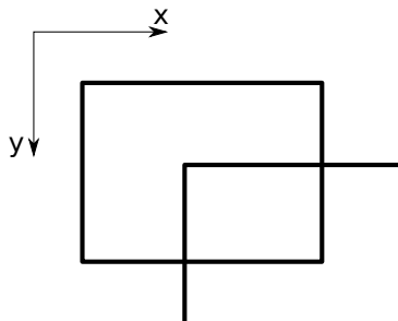
Figure 150: Example used in the AABB collision detection
